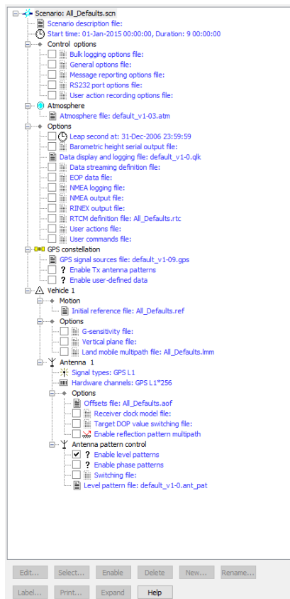
Figure 4 Scenario tree
